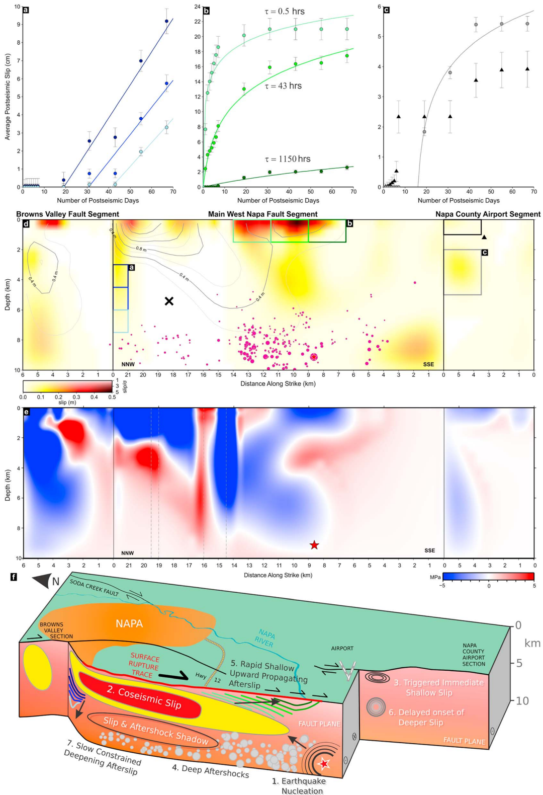
Figure 3. Variable behavior in time and space of afterslip and relationship of cumulative slip to coseismic Coulomb stress changes and aftershocks. (a–c) Temporal evolution of characteristic slip on patches of the fault. (d) Cumulative slip distribution across the model fault plane, where colored boxes correspond to the patches shown in the slip evolution time series, above. Segmentation of the model fault is as in Figures 1c and 2. (e) Coulomb stress change on the West Napa Fault plane due to modeled coseismic slip distribution (see Figure 1c), calculated using Coulomb 3 [Toda et al., 2005, 2011]. (f) Schematic summary of our findings, as described in the text, showing the sequence of slip behavior.
